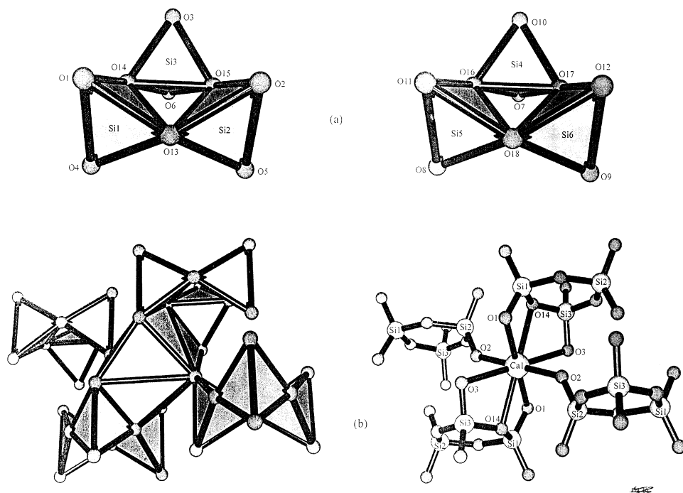
Fig. 10. Retrosynthesis of the crystal structure of pseudo-wollastonite \alpha - \text{CaSiO}_3 . (a) The two trimeric \text{Si}_3\text{O}_9 rings of corner-sharing \text{SiO}_4 tetrahedra. (b) Model cluster [\text{Ca}(\text{Si}_3\text{O}_9)_4]_{12} extracted from the network with an eight-fold coordinated calcium atom with both bidentate and tridentate coordination modes for the \text{Si}_3\text{O}_9 rings.
