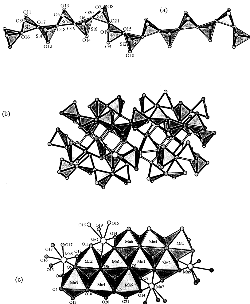
Fig. 7. Retrosynthesis of the crystal structure of pyroxmangite \text{MnSiO}_3 ( Z=28 ). (a) Linear chain of corner-sharing tetrahedra. (b) Model cluster [\text{Mn}_7\text{Si}_{21}\text{O}_{68}]^{26-} extracted from the pyroxmangite network. (c) Manganese–oxygen core of the model cluster evidencing the pivot atoms Mn5 and Mn7.
