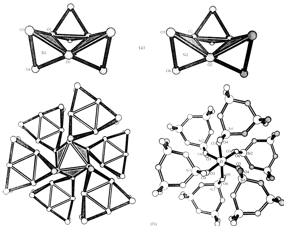
Fig. 12. Retrosynthesis of the crystal structure of wadeite K_2ZrSi_3O_9 . (a) The two trimeric Si_3O_9 ring of corner-sharing SiO_4 tetrahedra. (b) Model [Zr(Si_3O_9)_6]^{32-} cluster extracted from the network with monodentate coordination mode for the Si_3O_9 rings [cf. Fig. 11(b) for the change in conformation].
